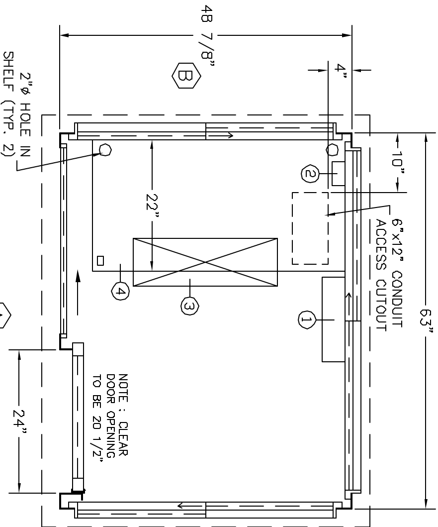
PLAN VIEW
