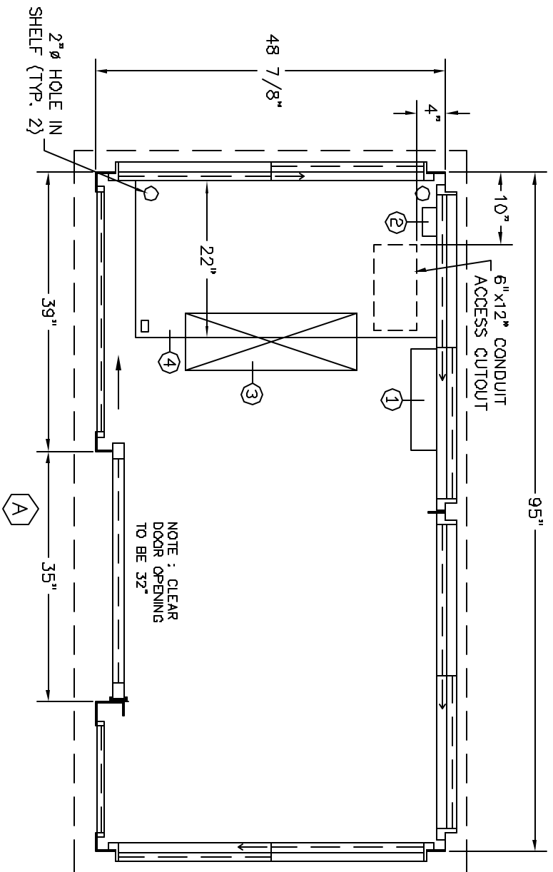
PLAN VIEW
