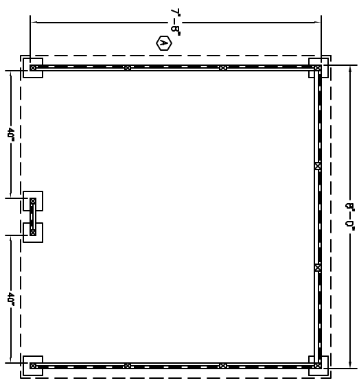
PLAN VIEW - STYLE "C"
