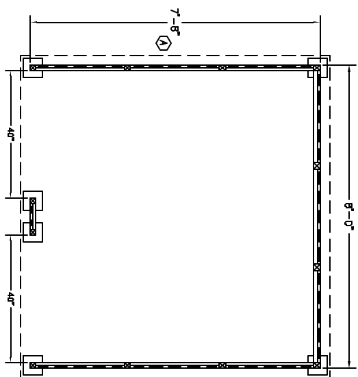
PLAN VIEW - STYLE "C"
