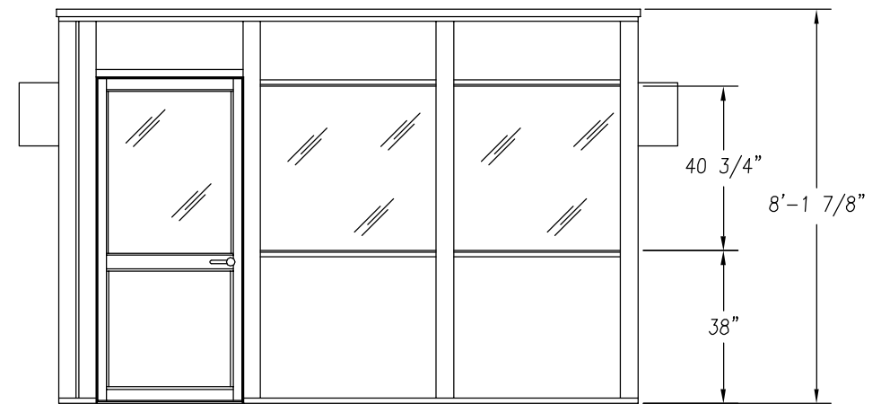
ELEVATION C
