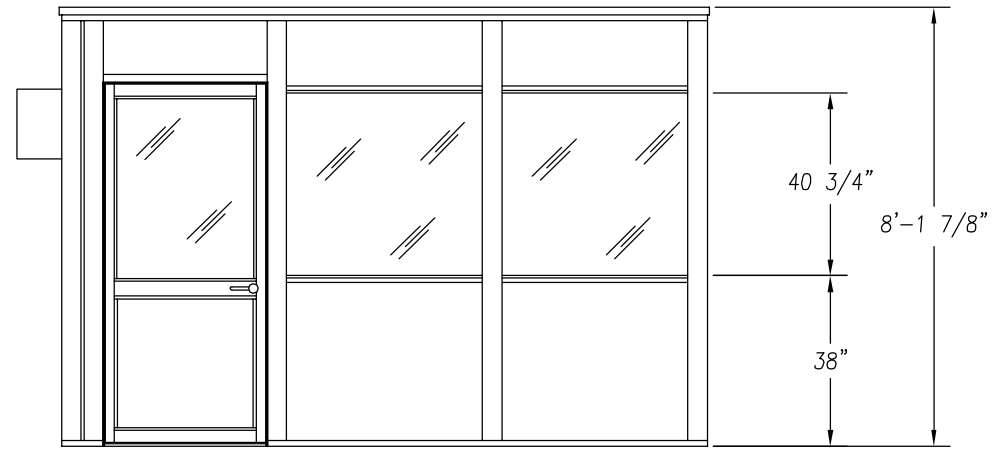
ELEVATION C
