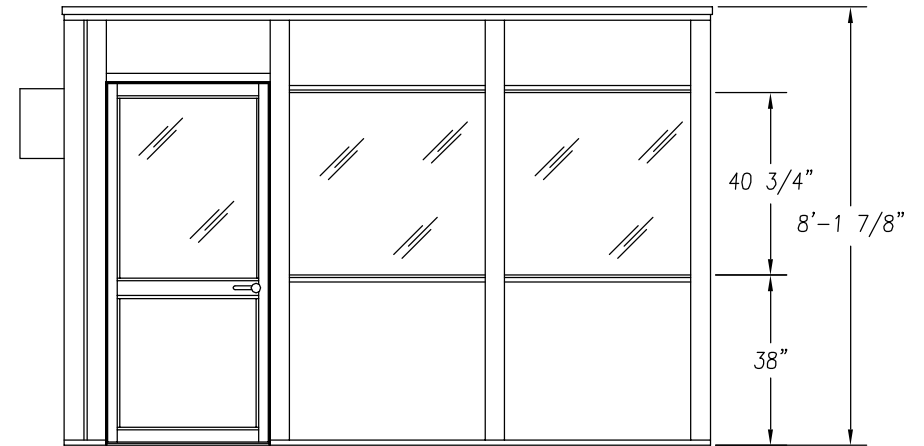
ELEVATION C
