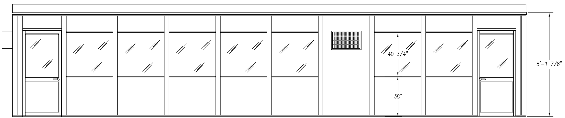
ELEVATION C
