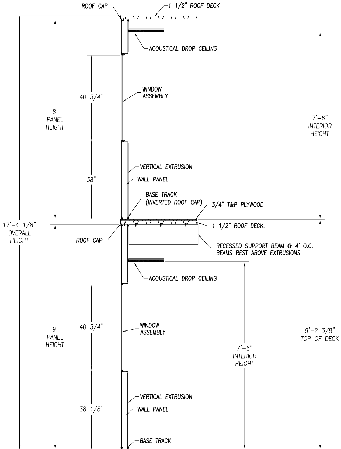
WALL SECTION
