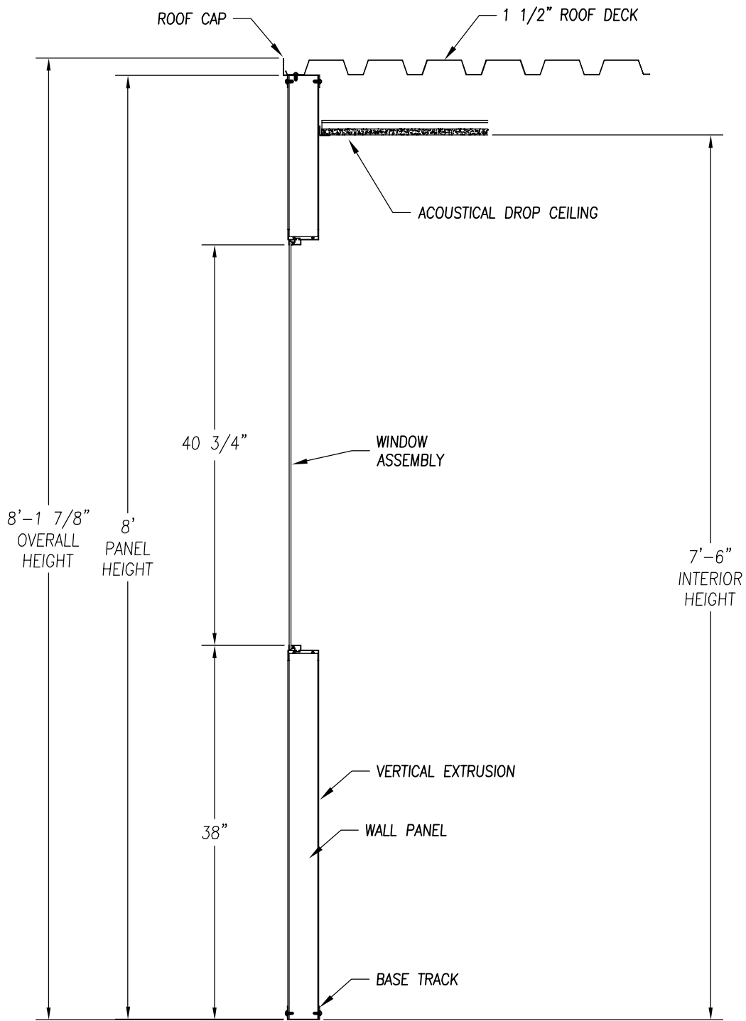
WALL SECTION
