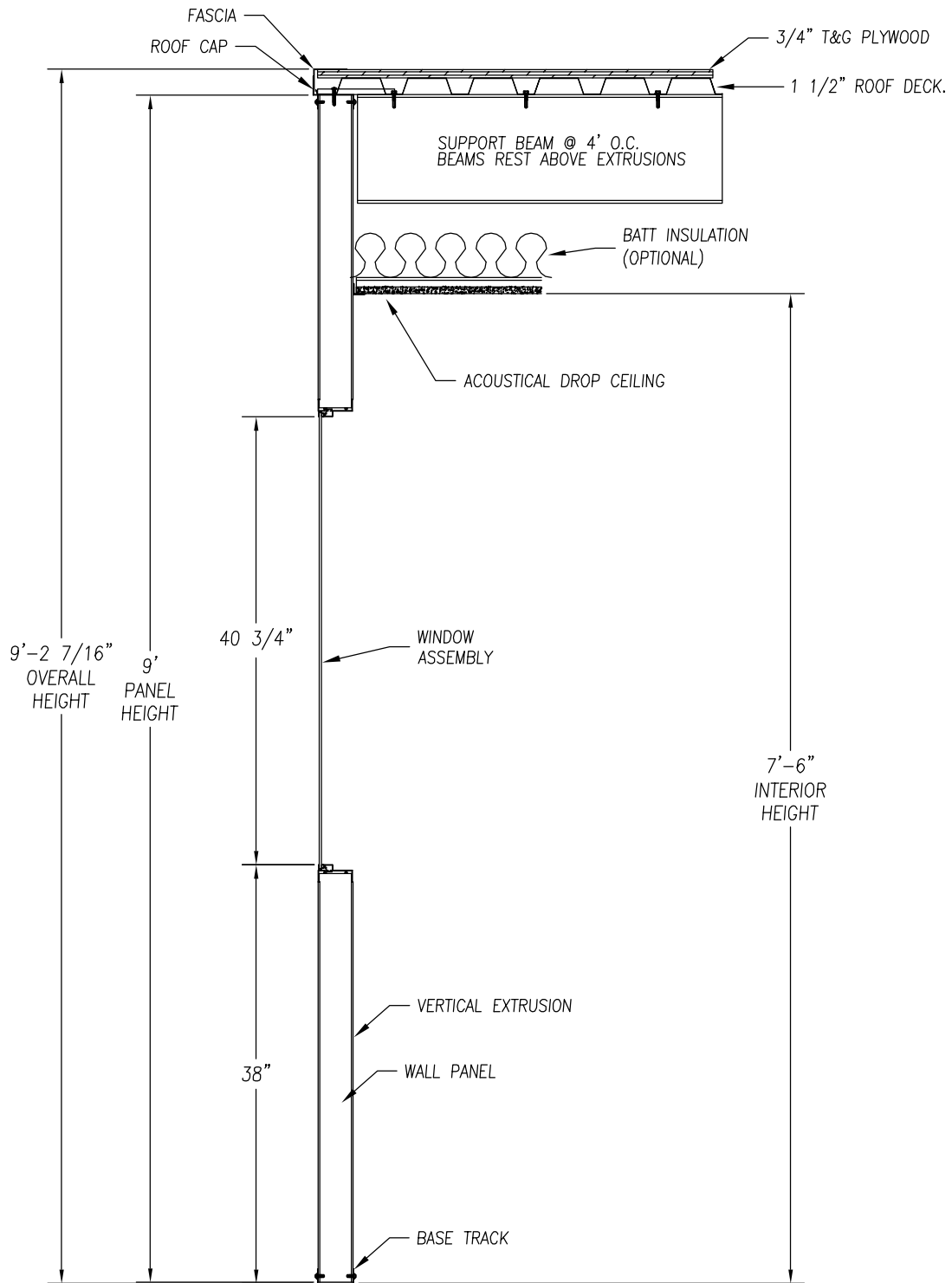
WALL SECTION
