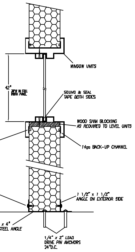
WINDOW SECTION
