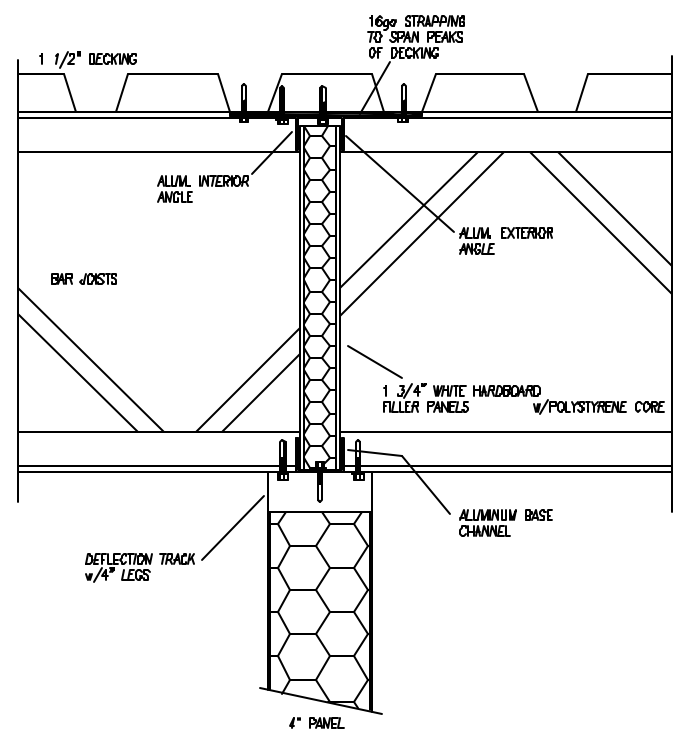
TOP SECTION
