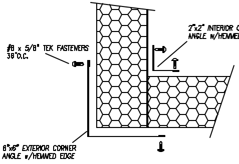
CORNER JOINT CONNECTION
