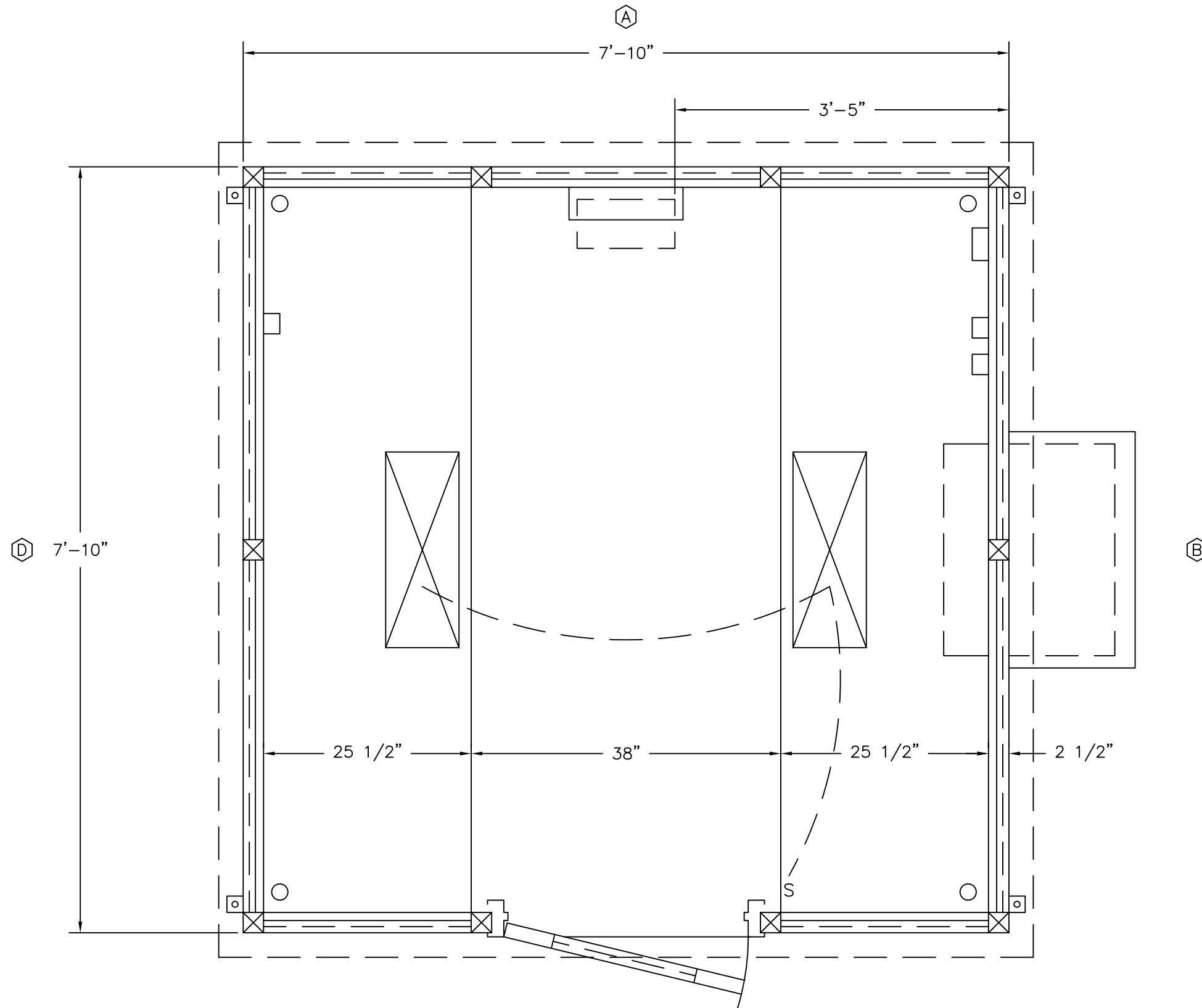
PLAN VIEW
