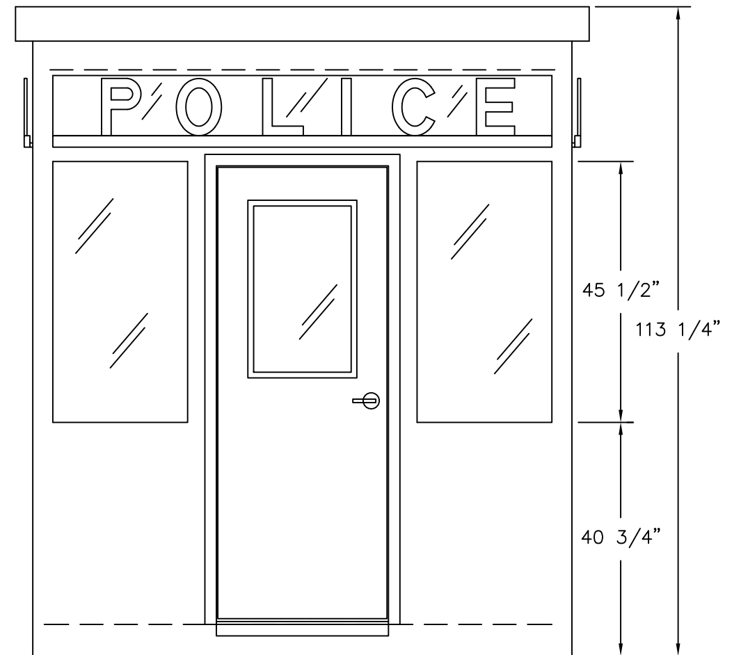
ELEVATION C
