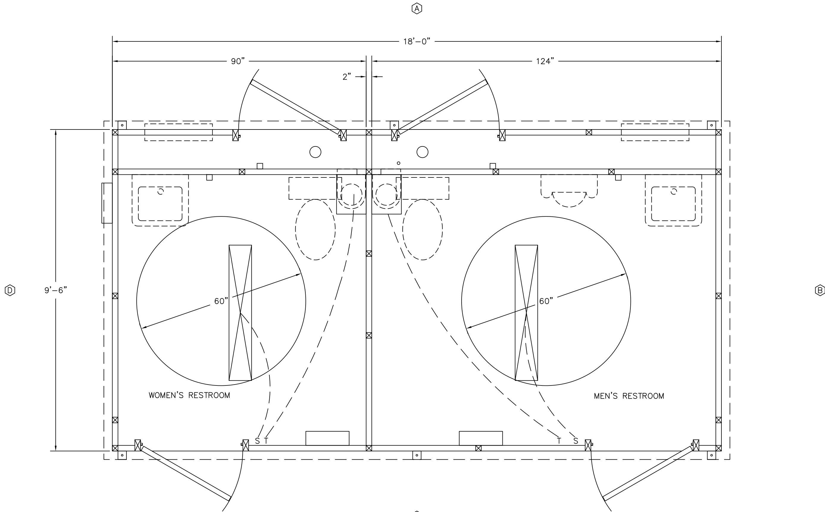
(C) PLAN VIEW
