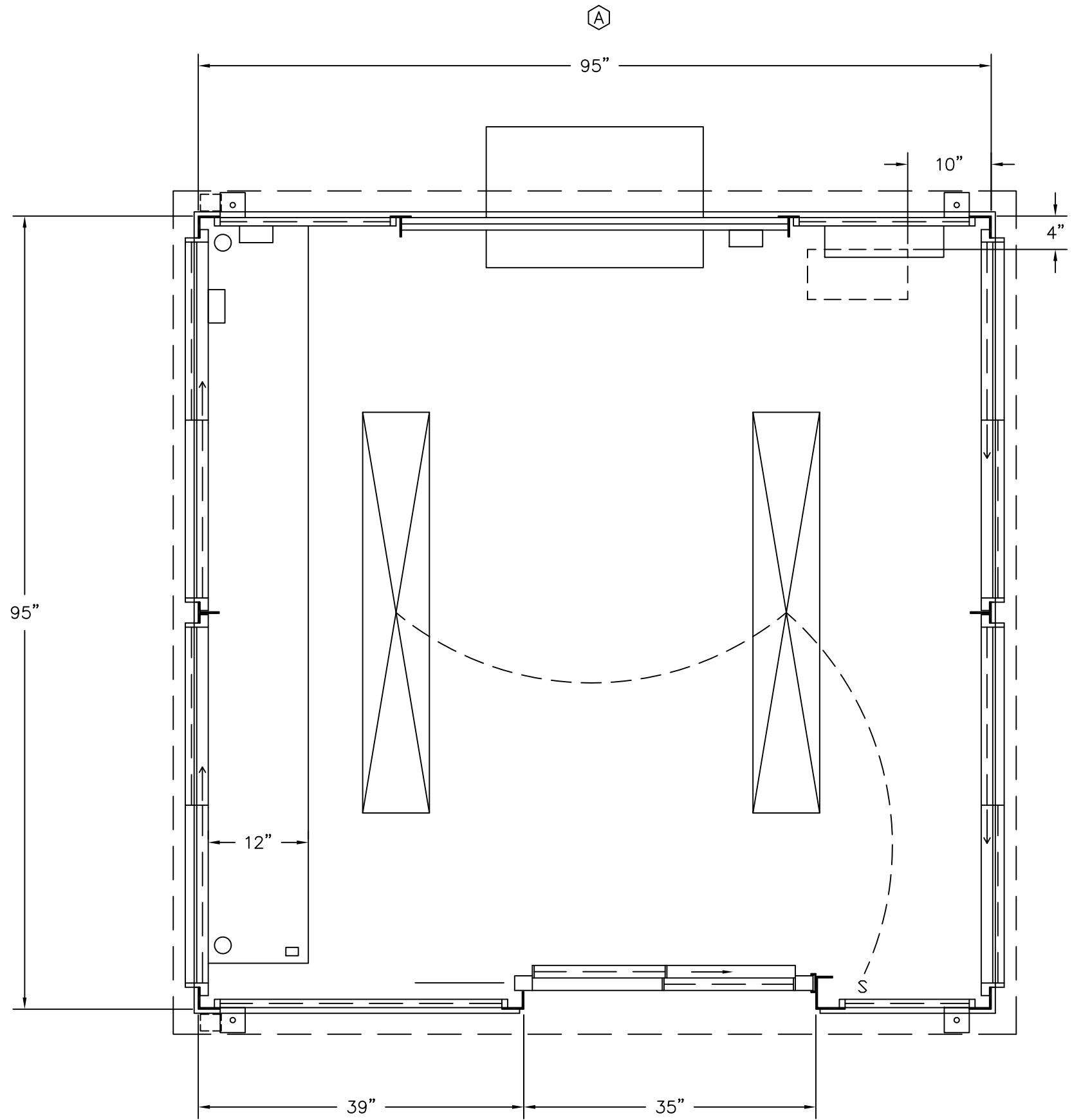
PLAN VIEW
