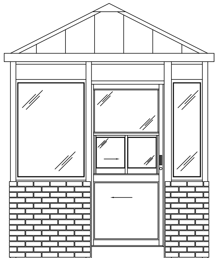
ELEVATION C
