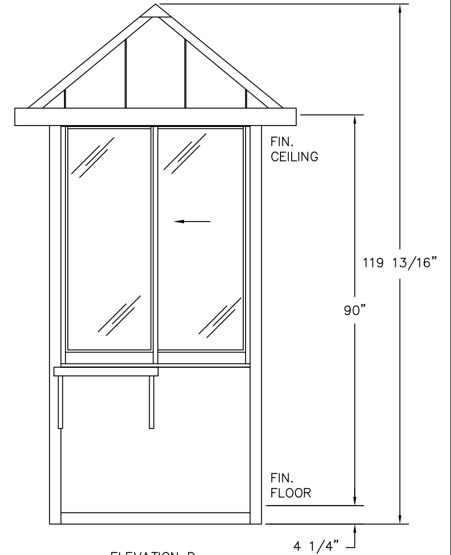
ELEVATION D
