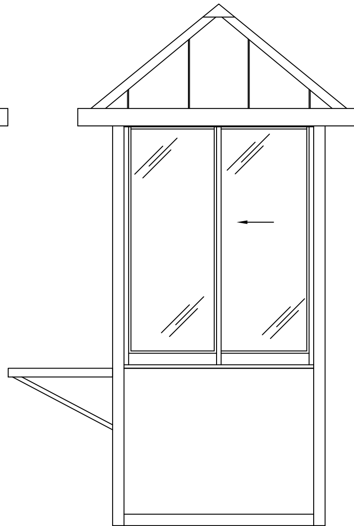
ELEVATION C
