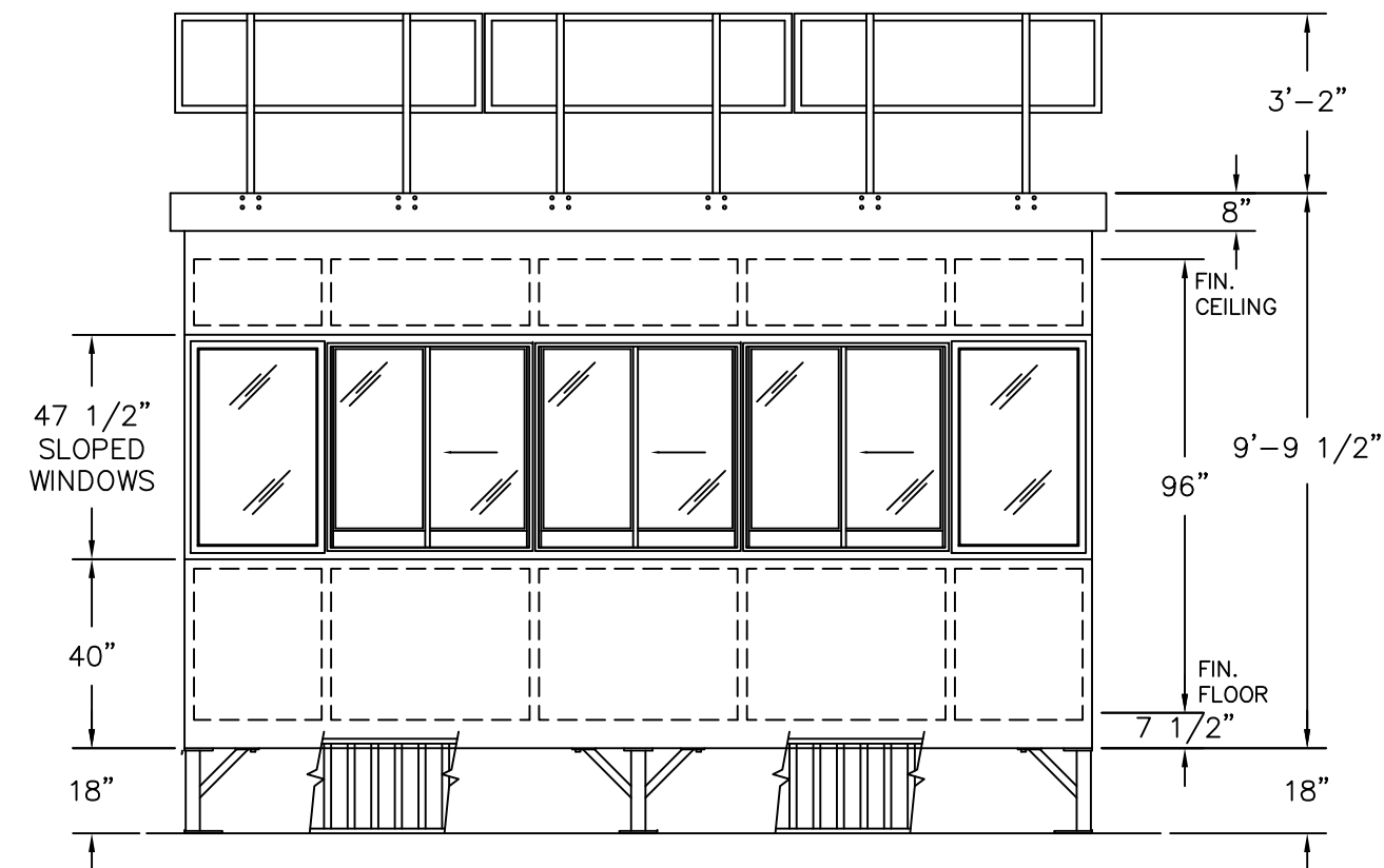
ELEVATION C
