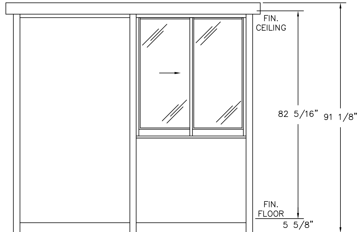
ELEVATION D
