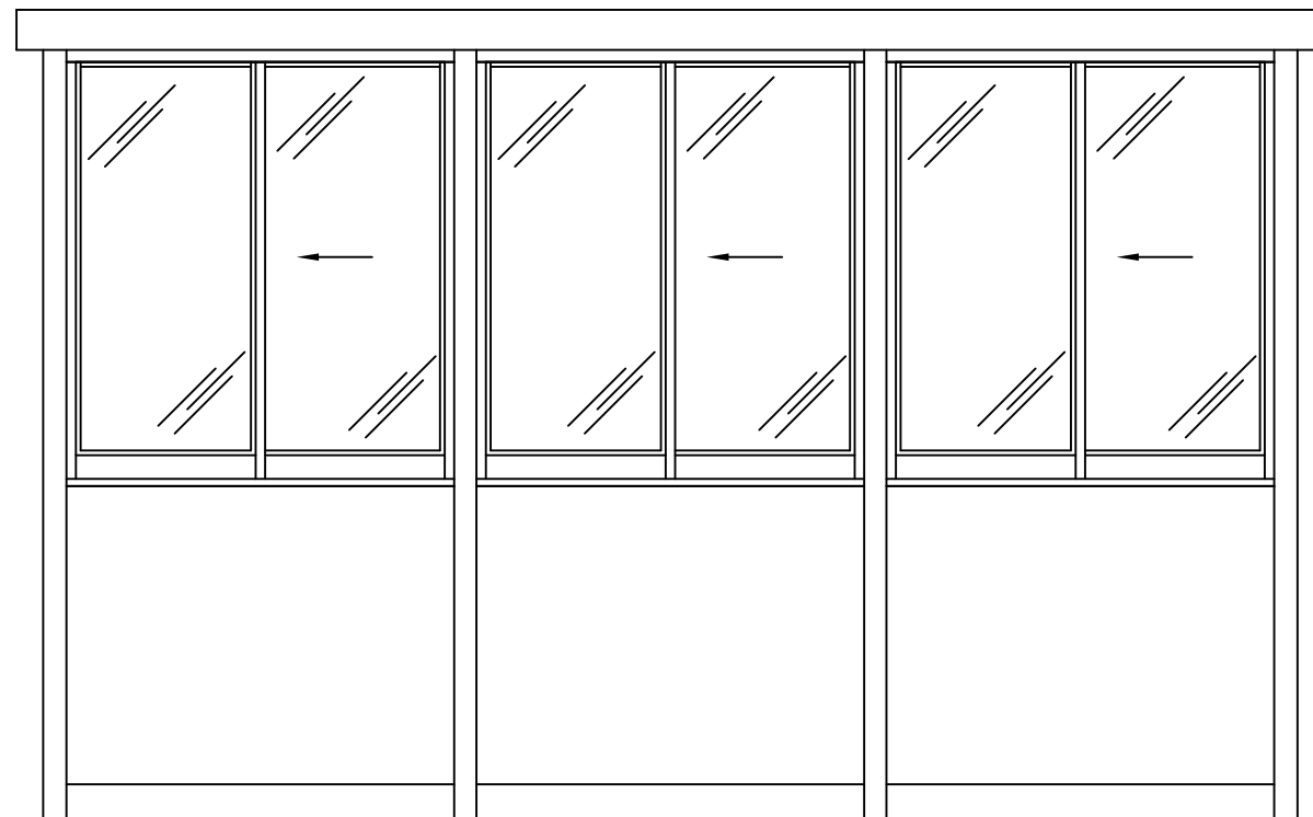
ELEVATION C
