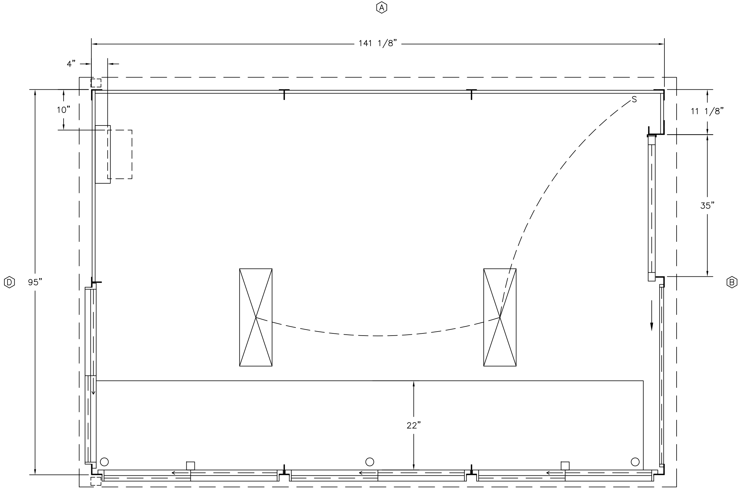
PLAN VIEW
