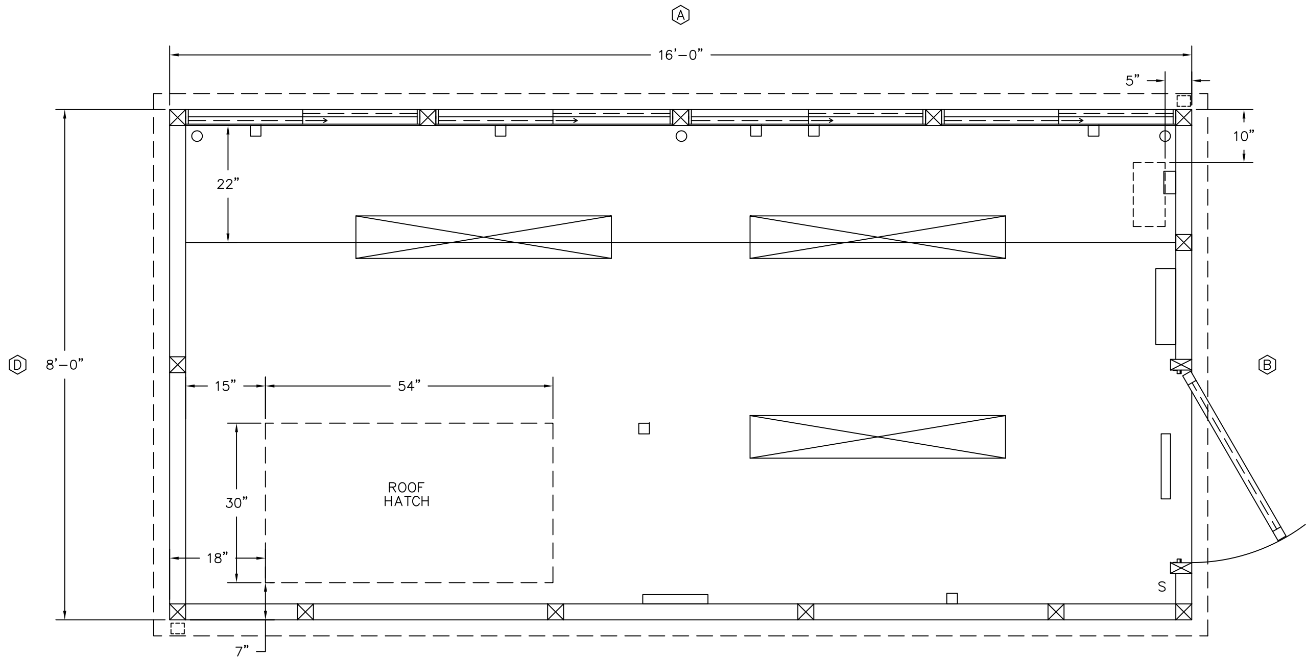
PLAN VIEW
