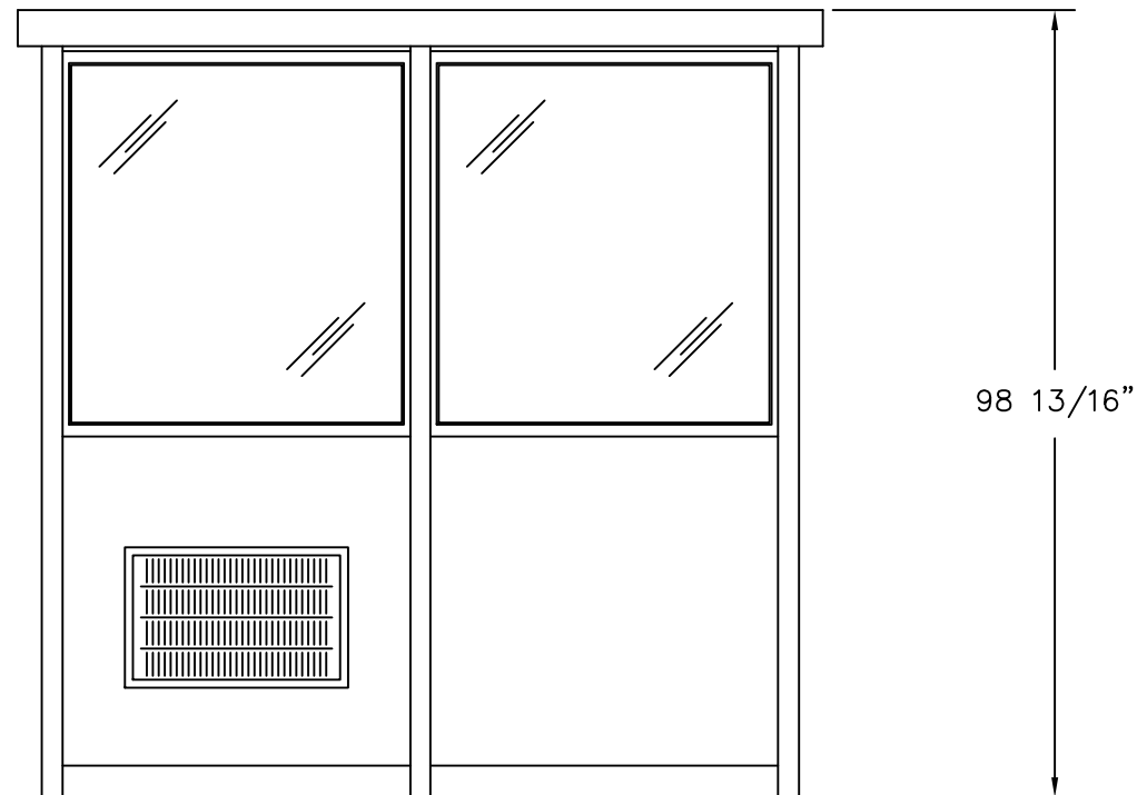
ELEVATION D
