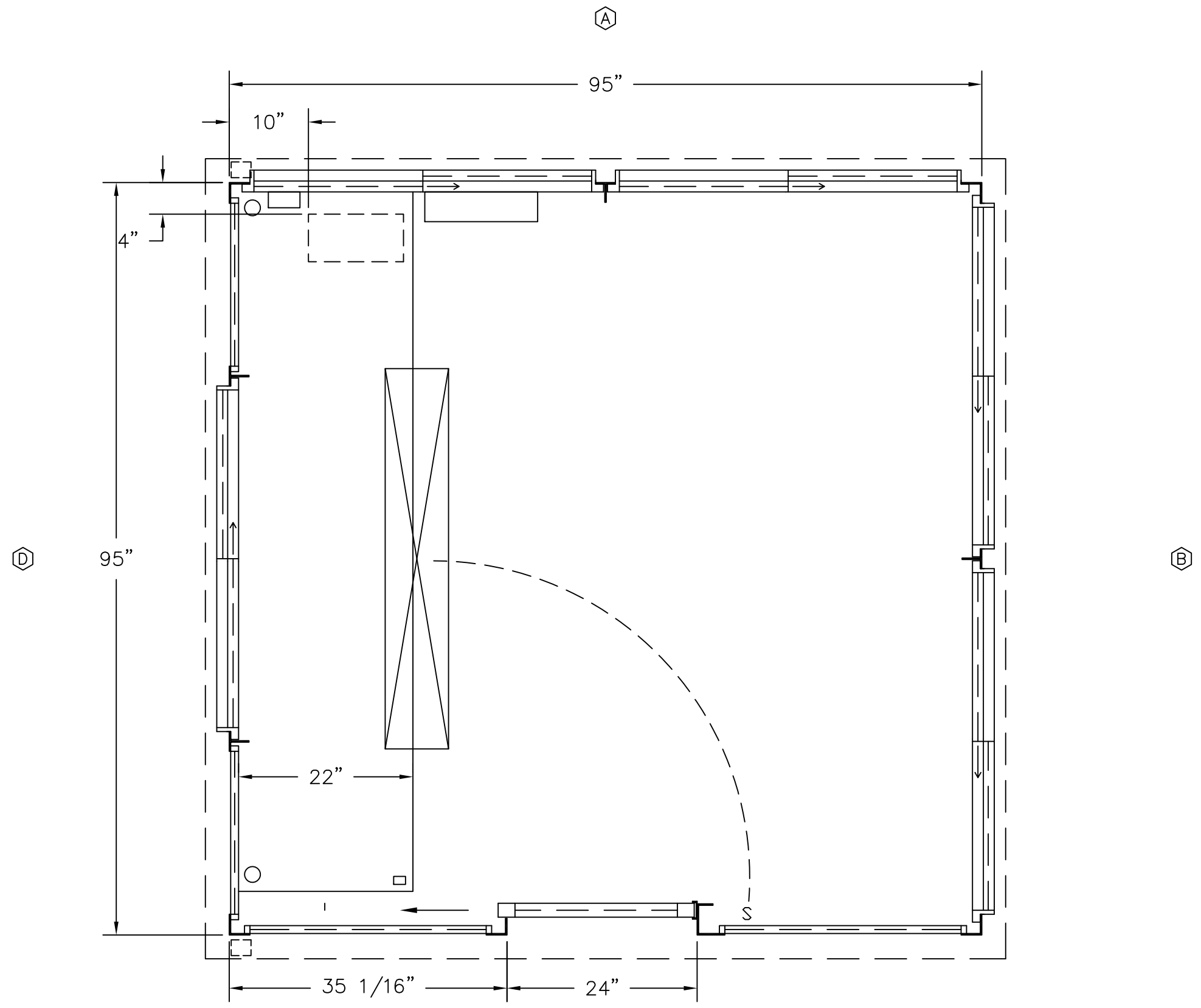
(C) PLAN VIEW
