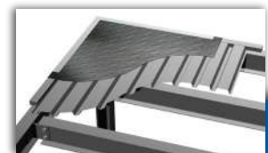
Checker plate and roof deck
