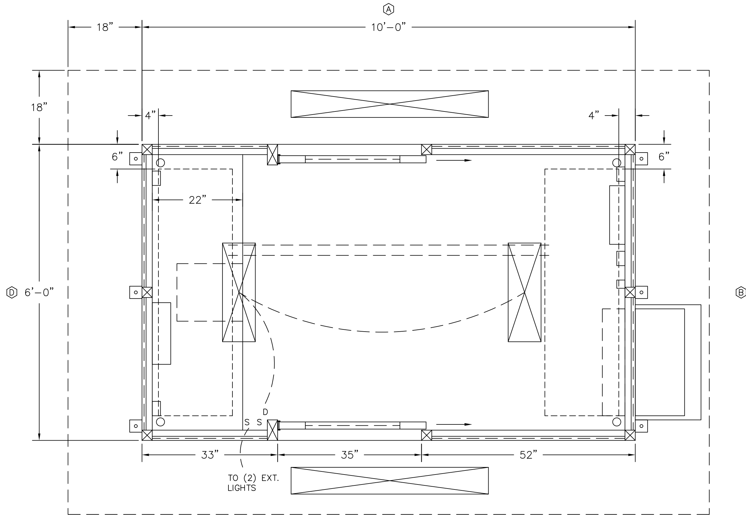
PLAN VIEW
