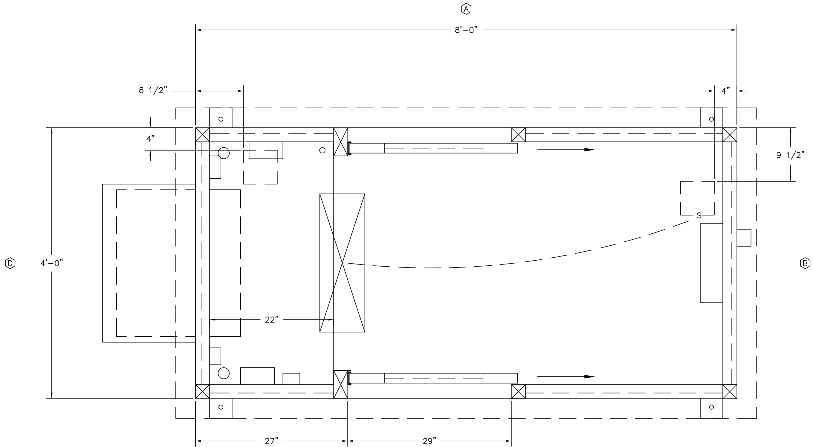
PLAN VIEW
