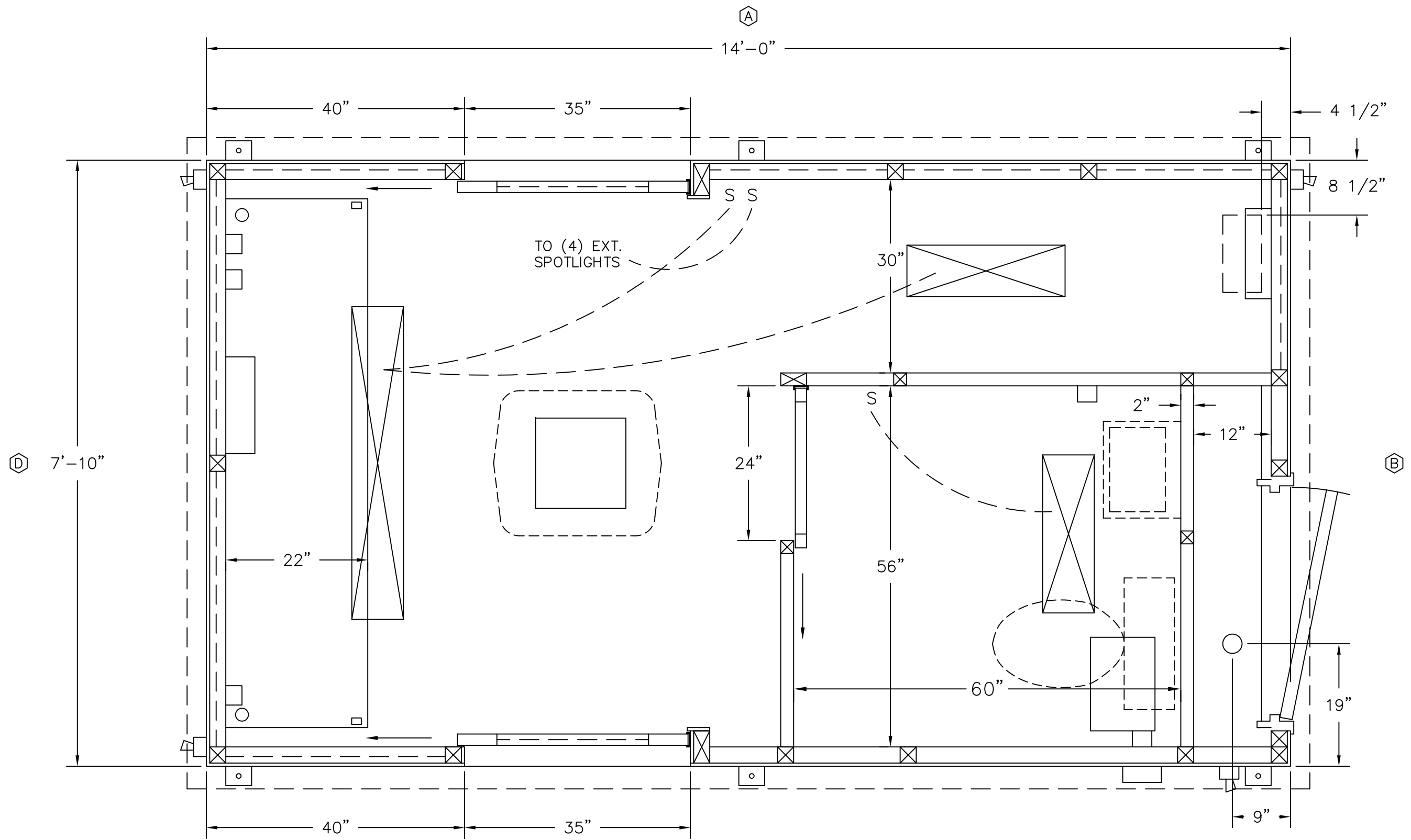
PLAN VIEW
