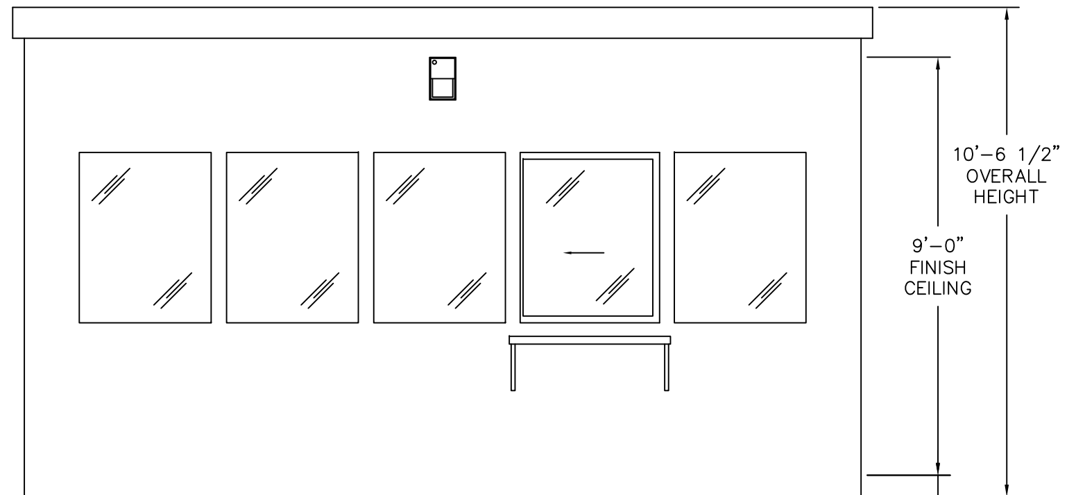
ELEVATION D
