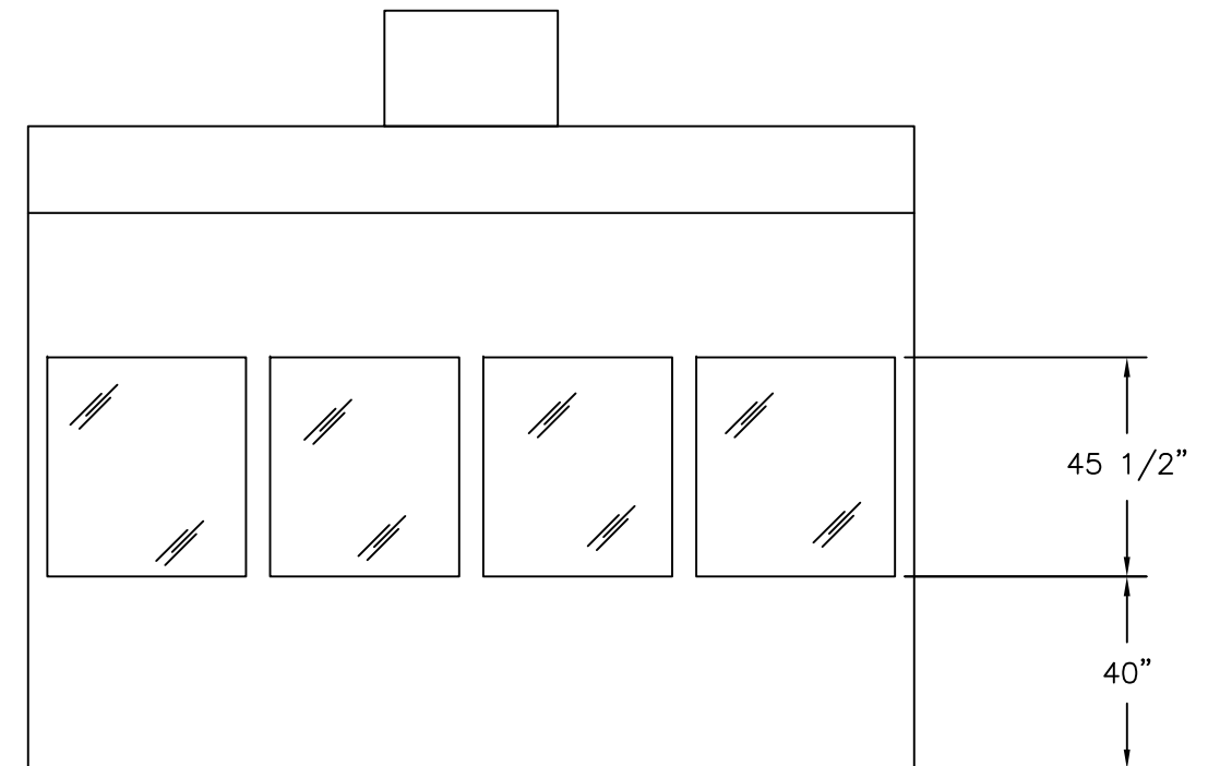
ELEVATION D
