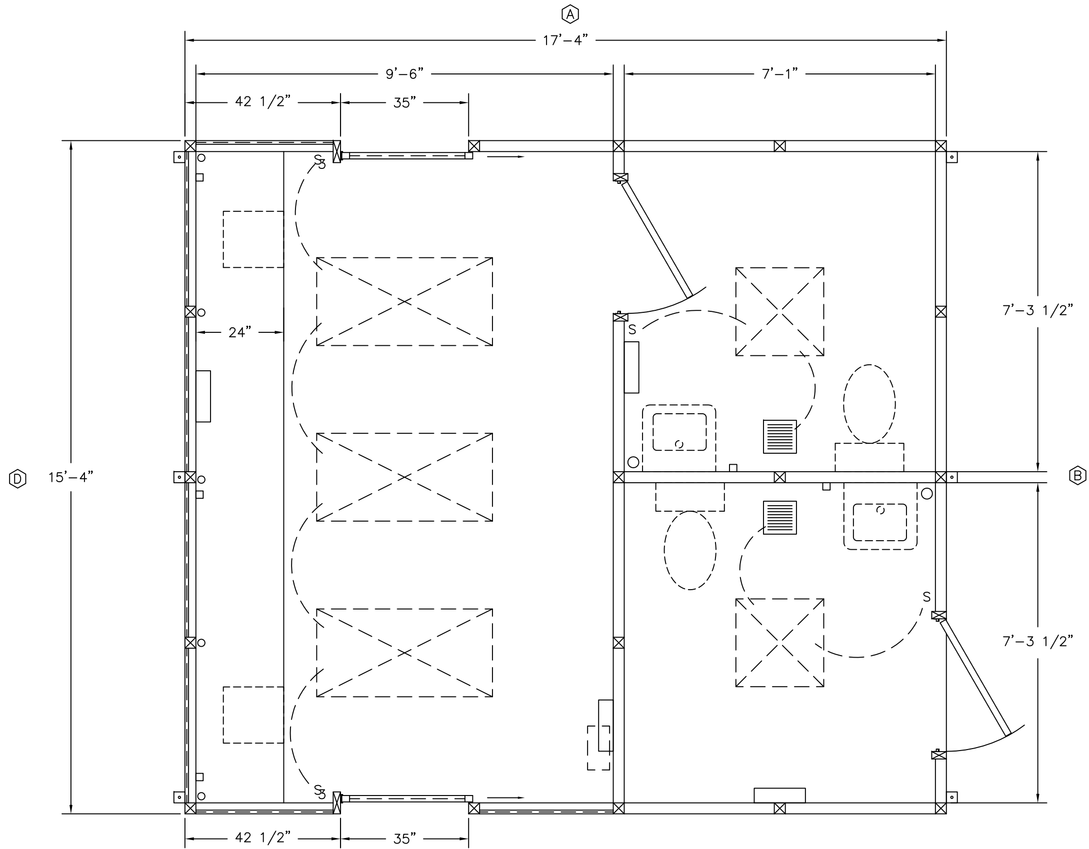
PLAN VIEW
