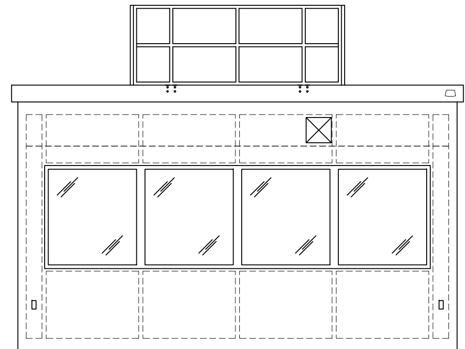
ELEVATION D
