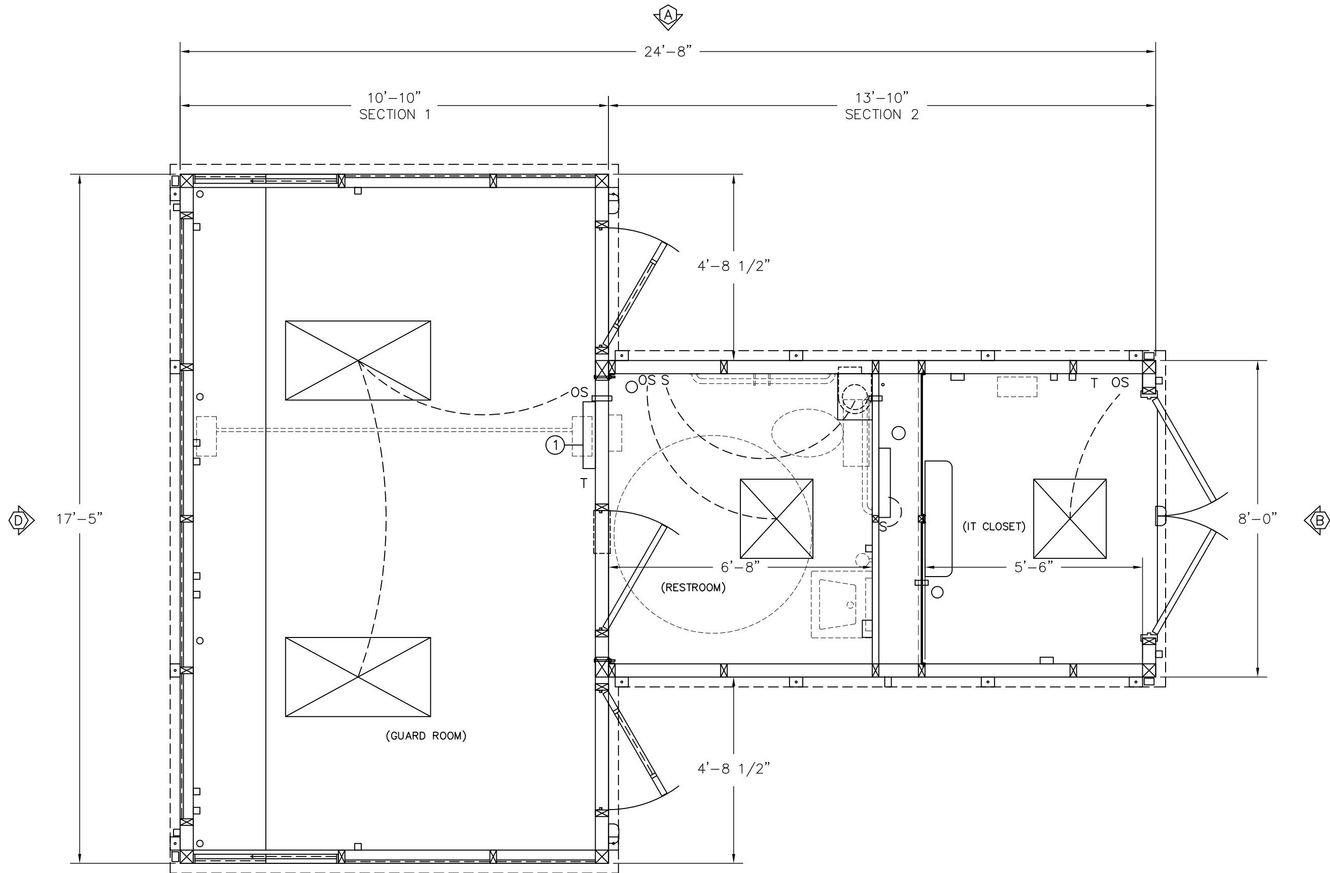
PLAN VIEW
