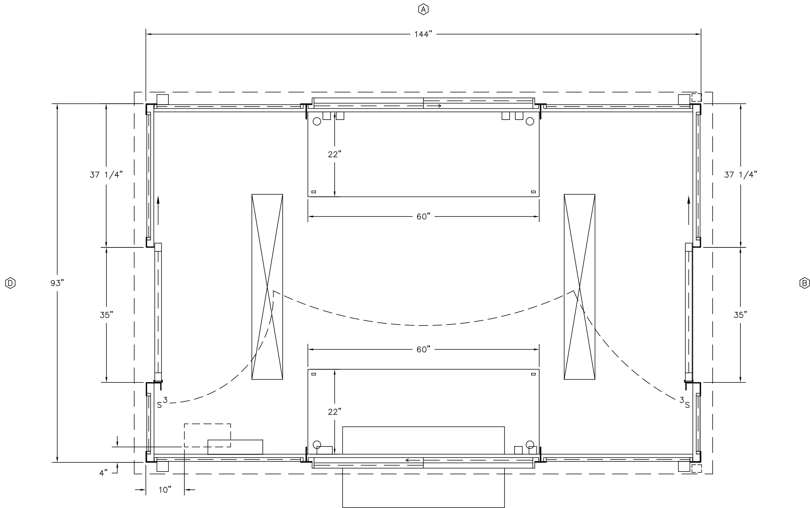
PLAN VIEW
