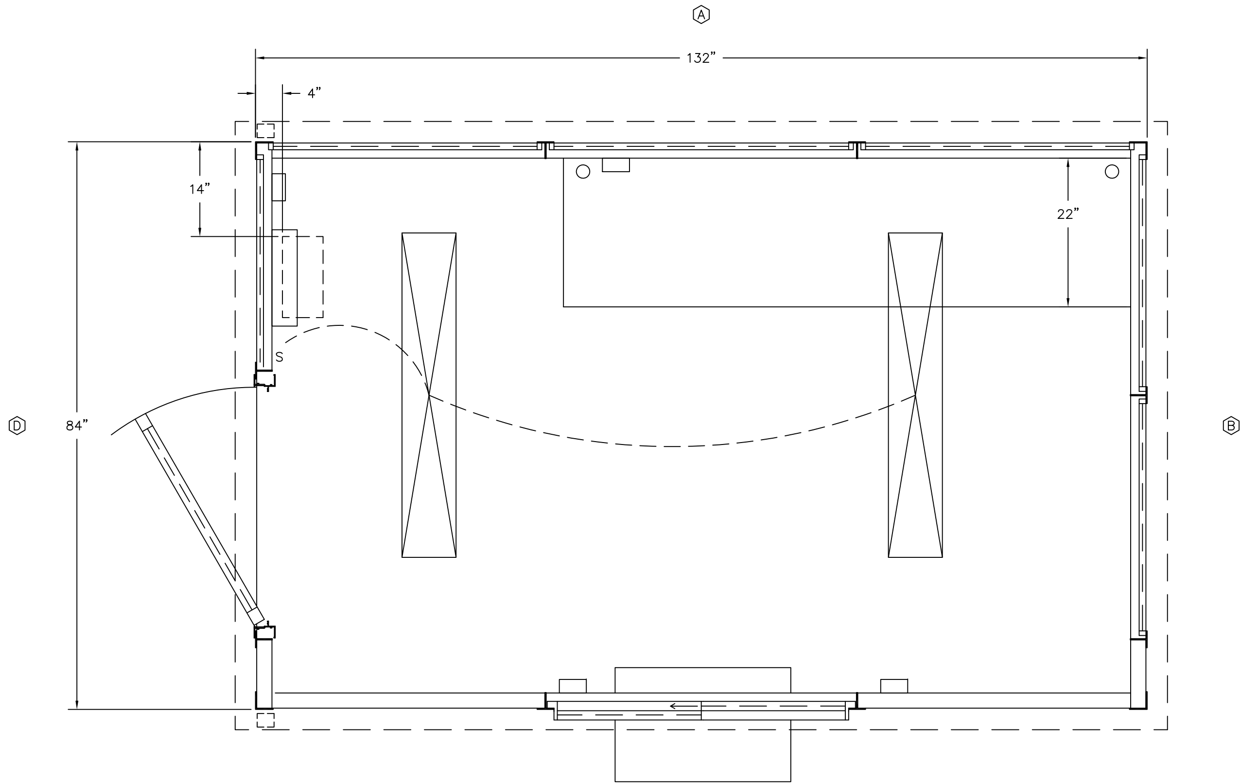
PLAN VIEW
