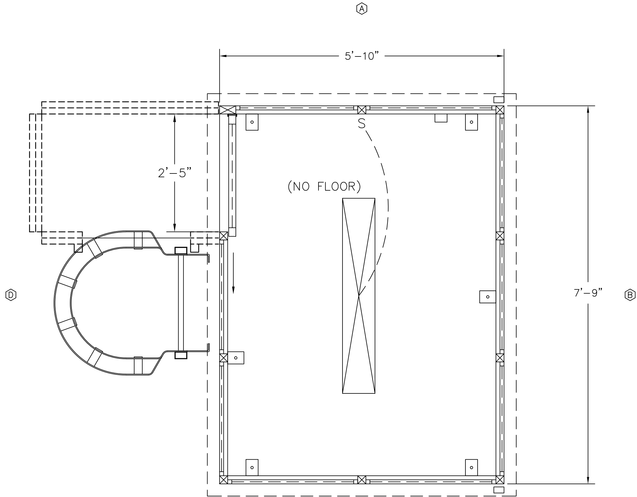
(C) PLAN VIEW
