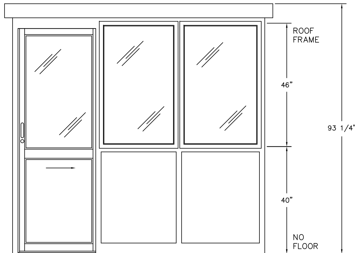
ELEVATION D
