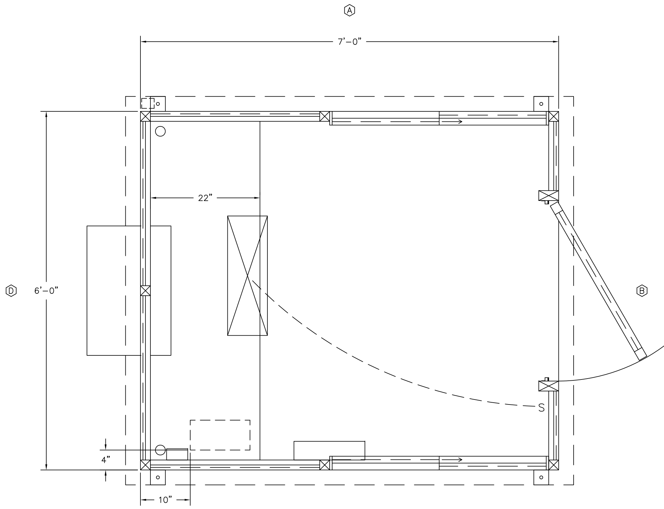
PLAN VIEW
