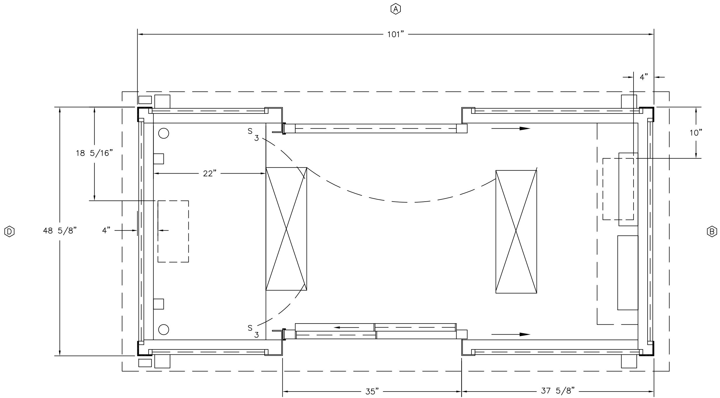
PLAN VIEW
