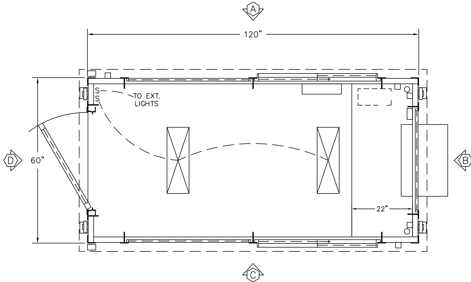
PLAN VIEW
