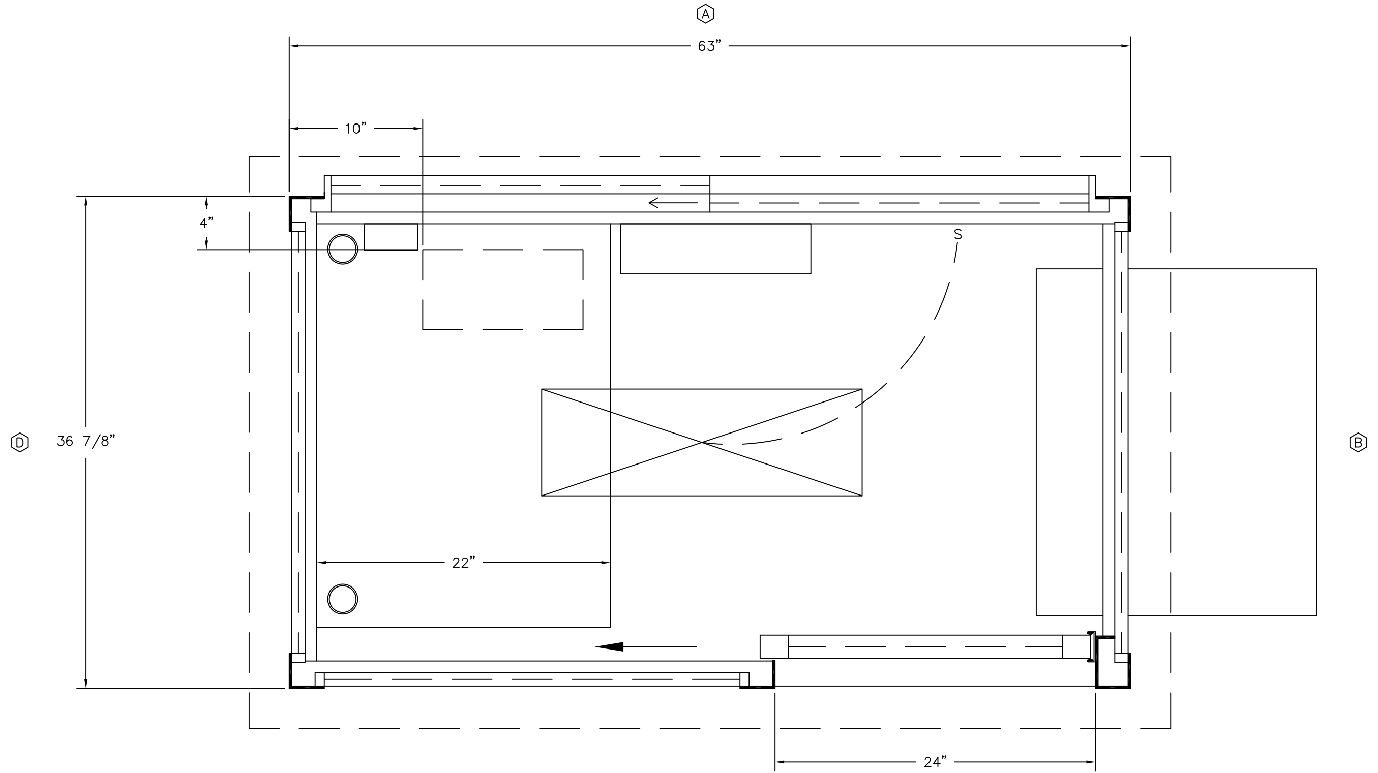
PLAN VIEW
