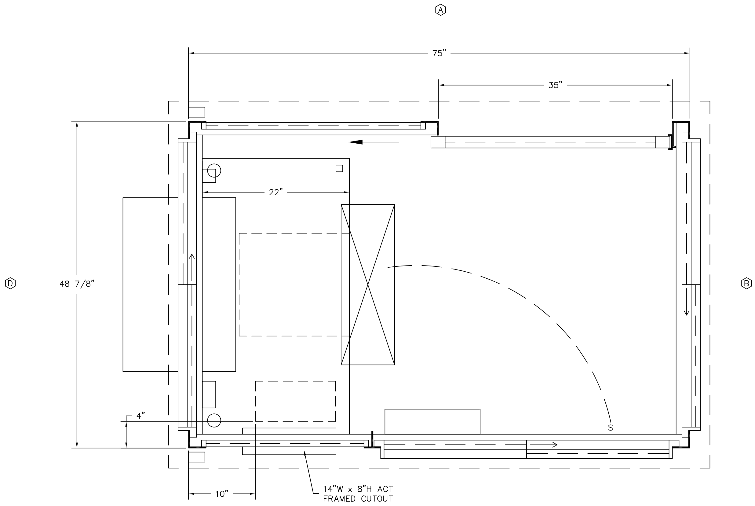
(C) PLAN VIEW
