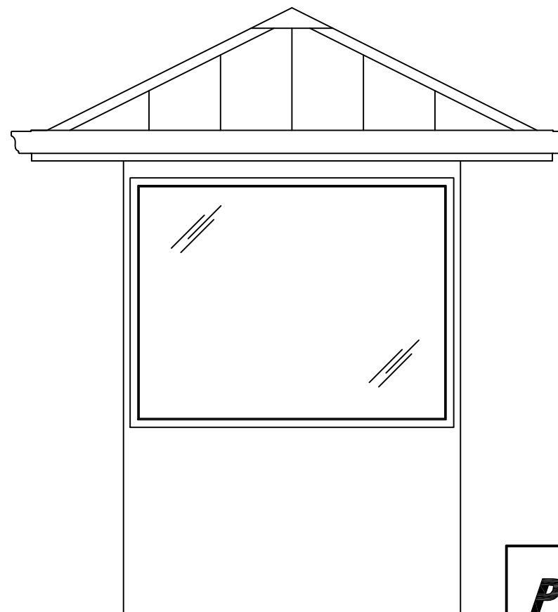
ELEVATION D
