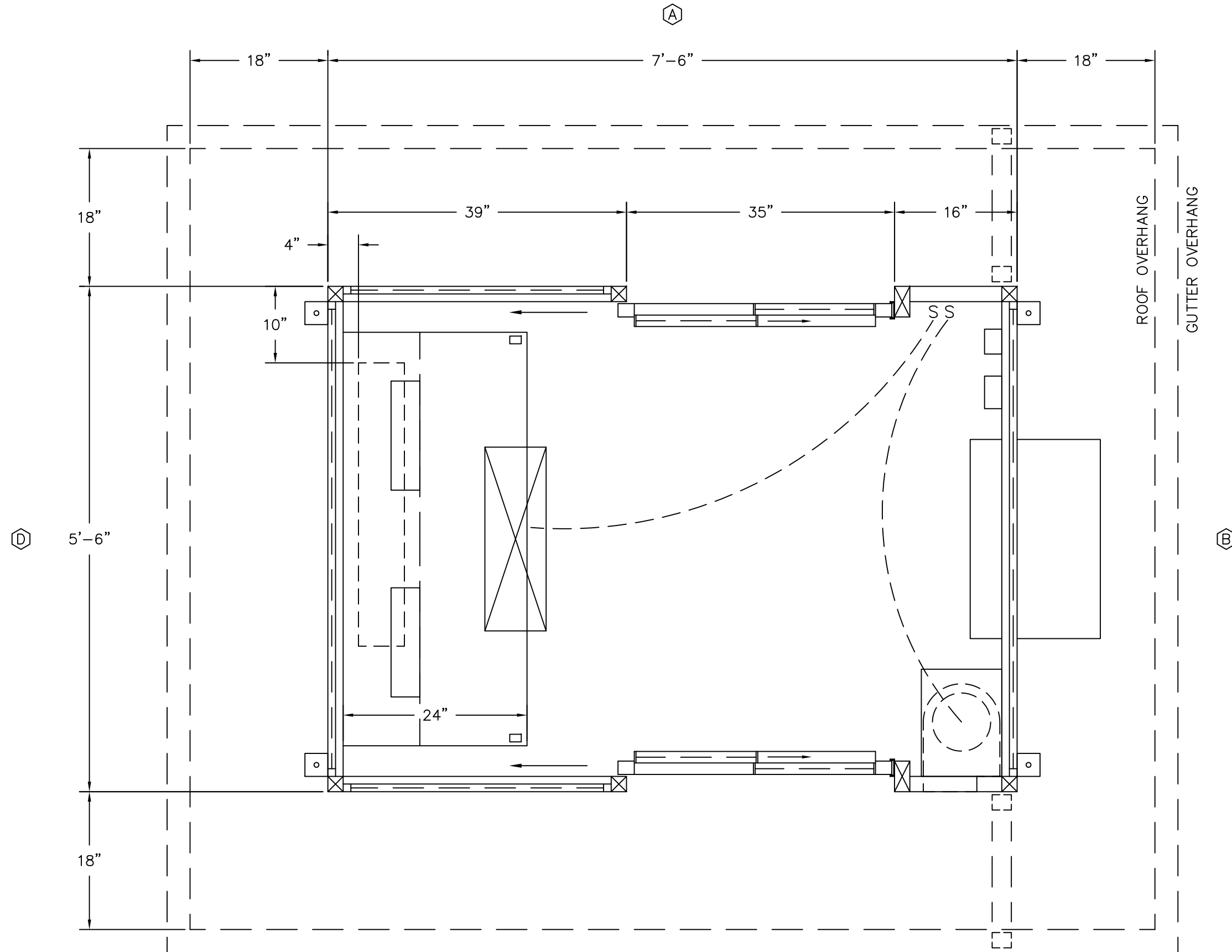
PLAN VIEW
