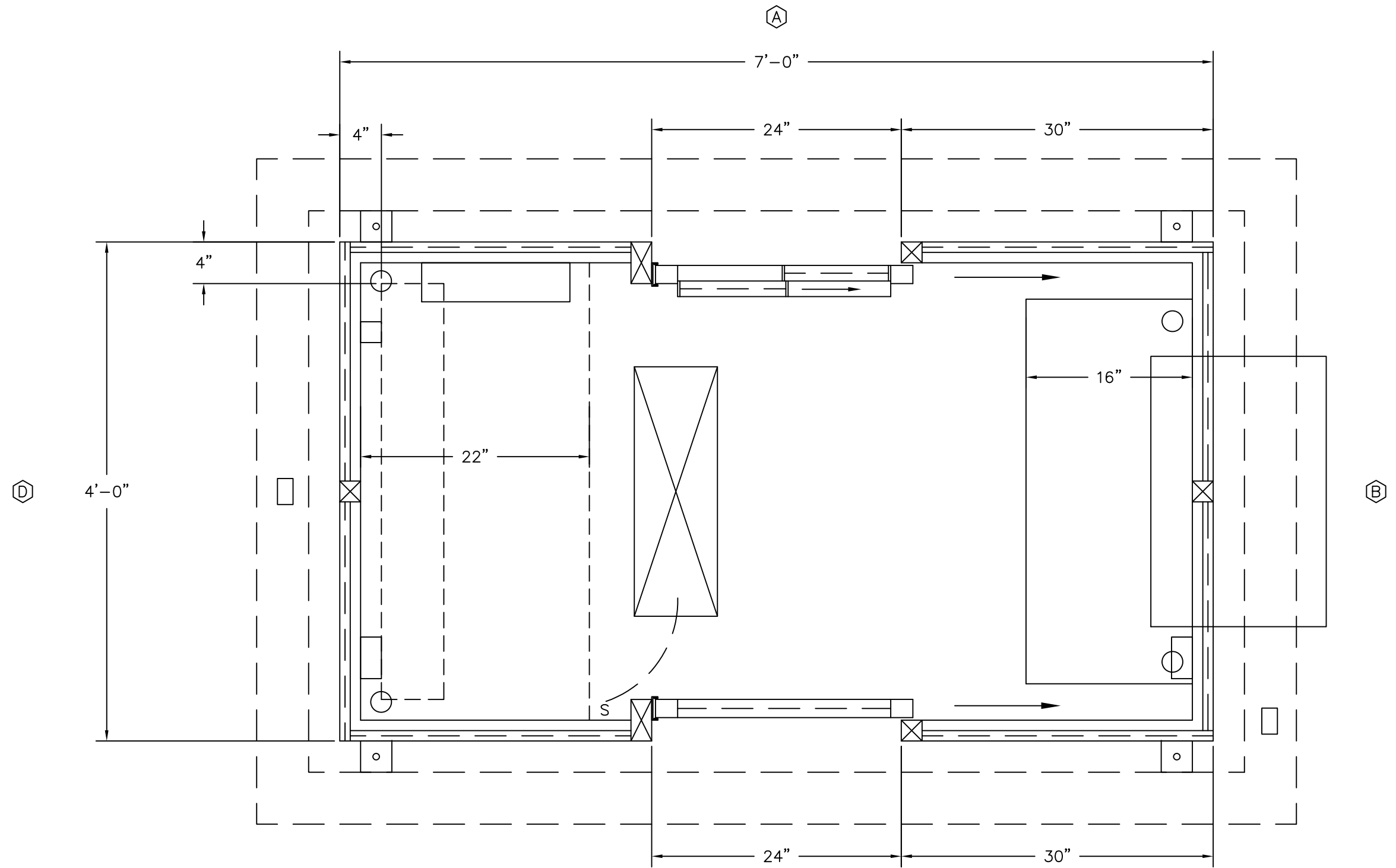
(C) PLAN VIEW
