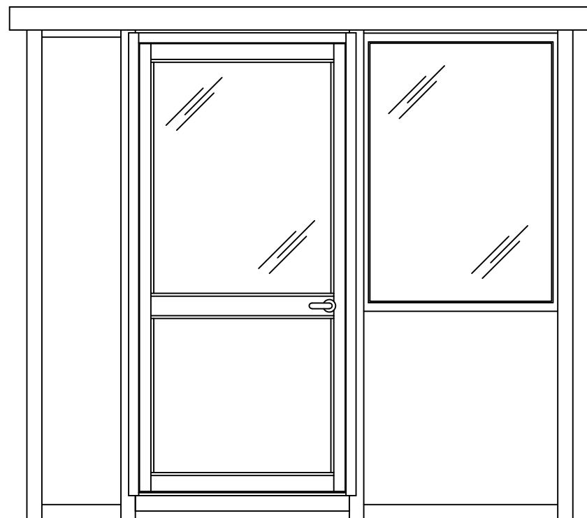
ELEVATION C
