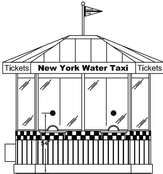
ELEVATION C
