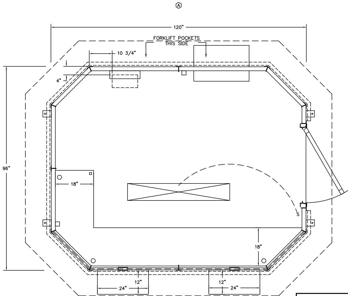
PLAN VIEW
