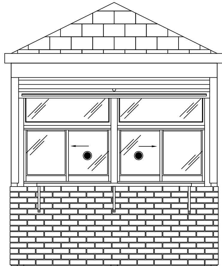
ELEVATION C
