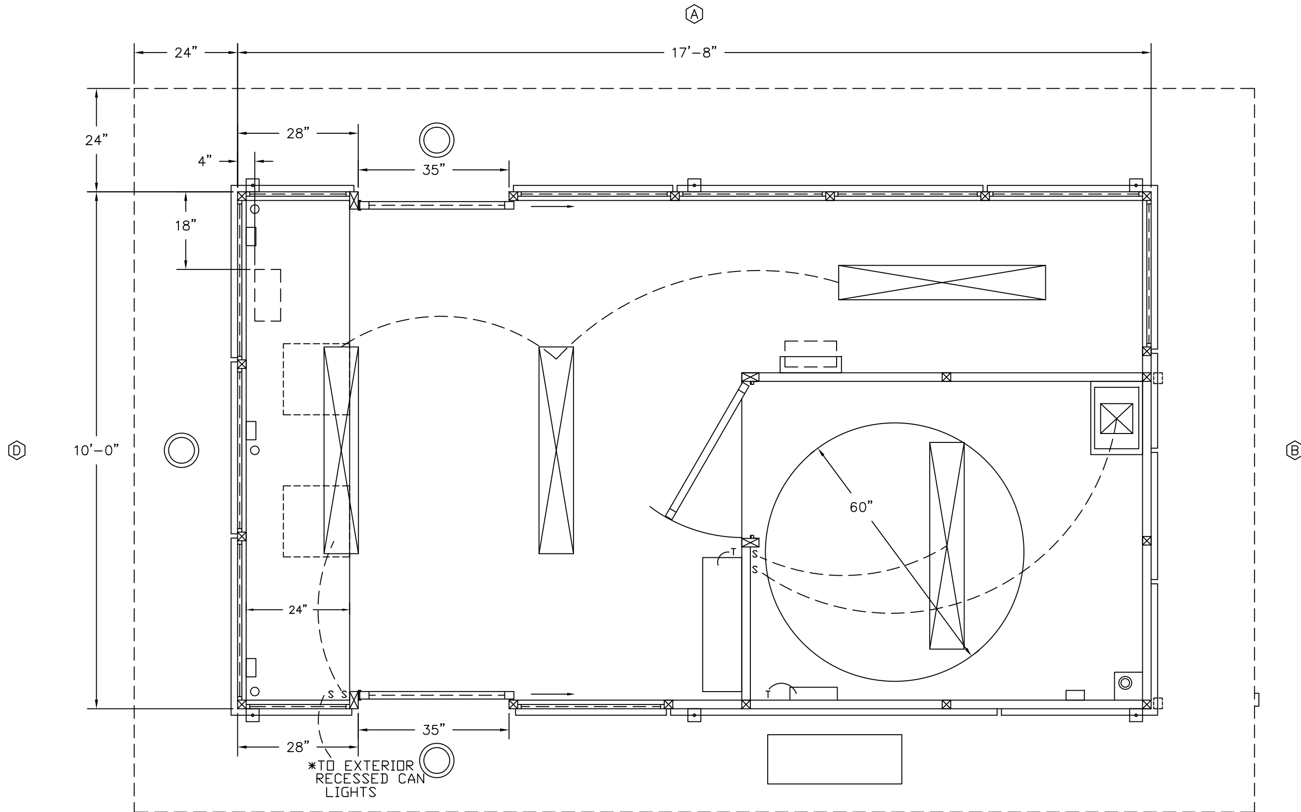
PLAN VIEW
