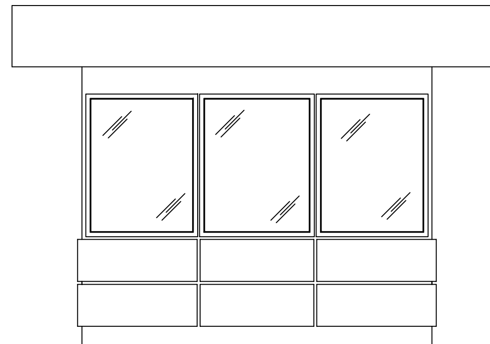
ELEVATION D
