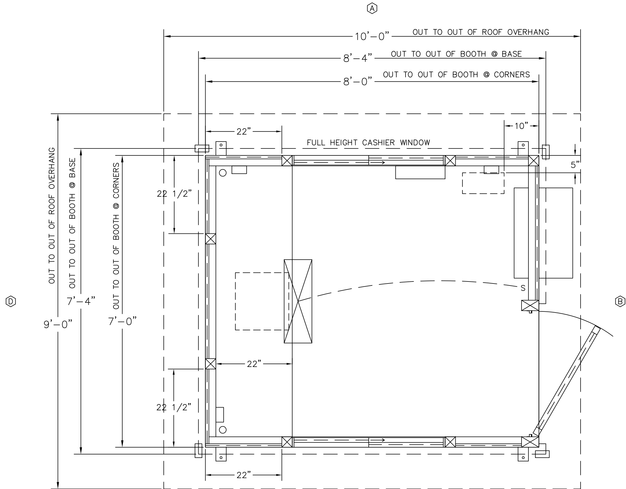
PLAN VIEW
