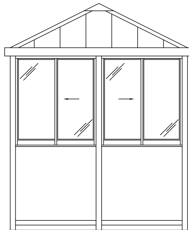
ELEVATION D
