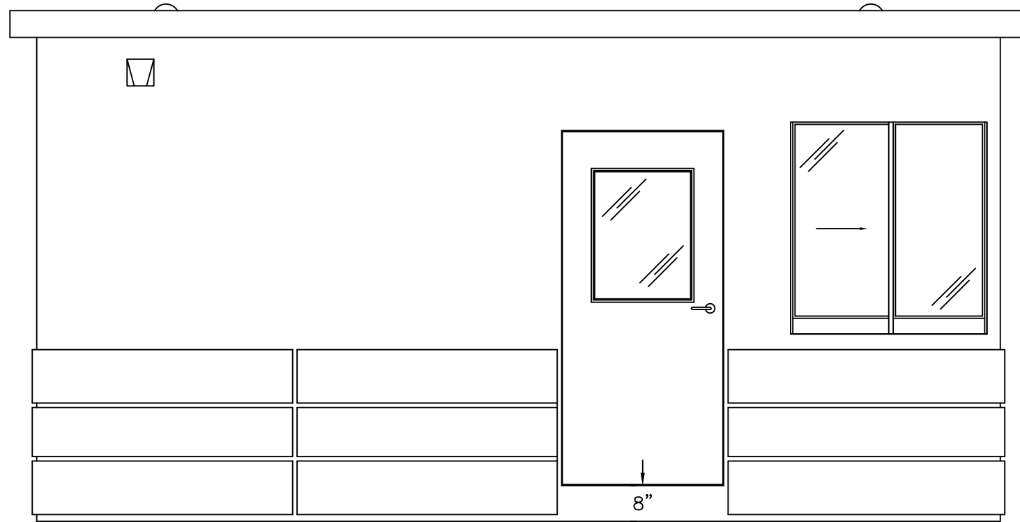
ELEVATION C
