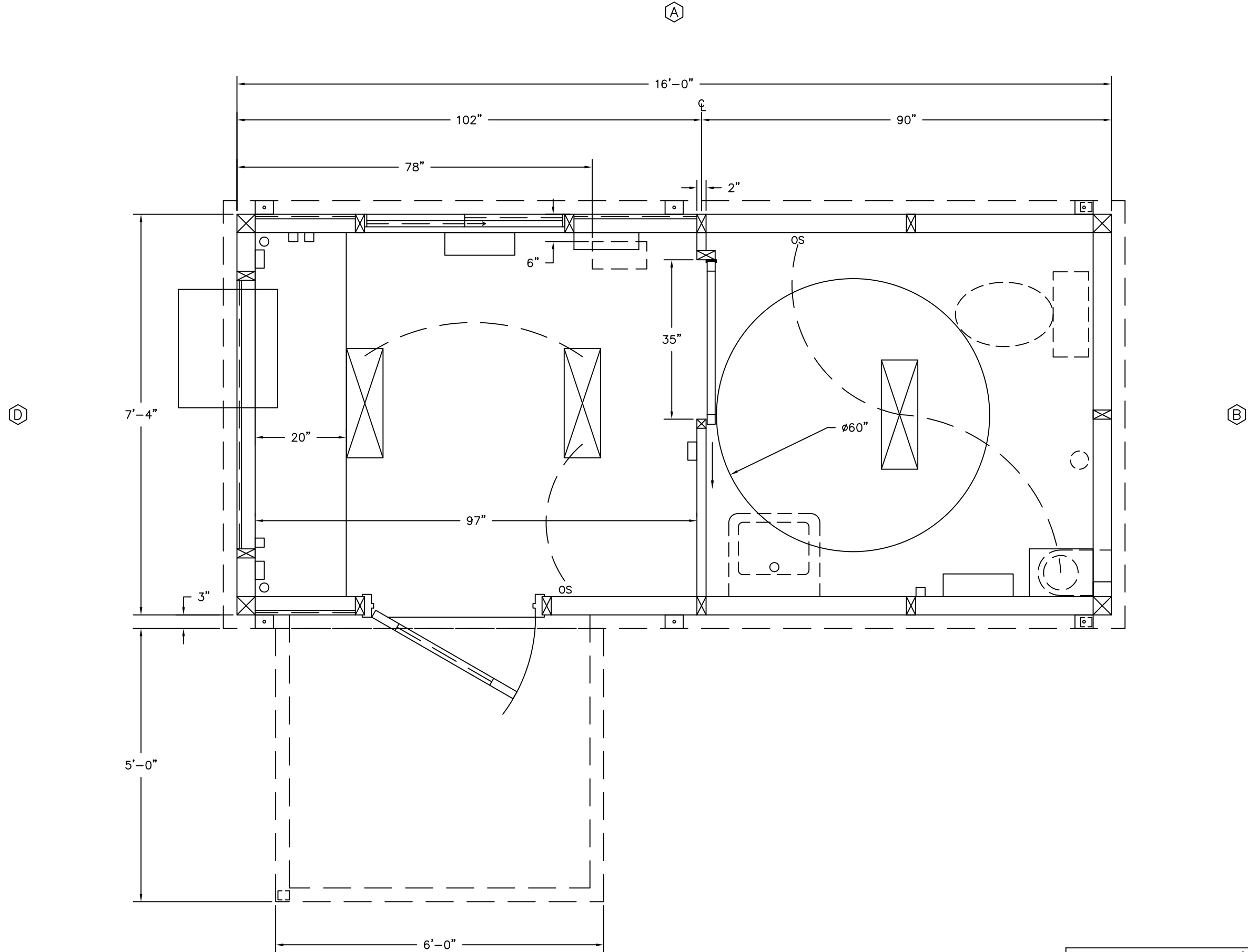
PLAN VIEW
