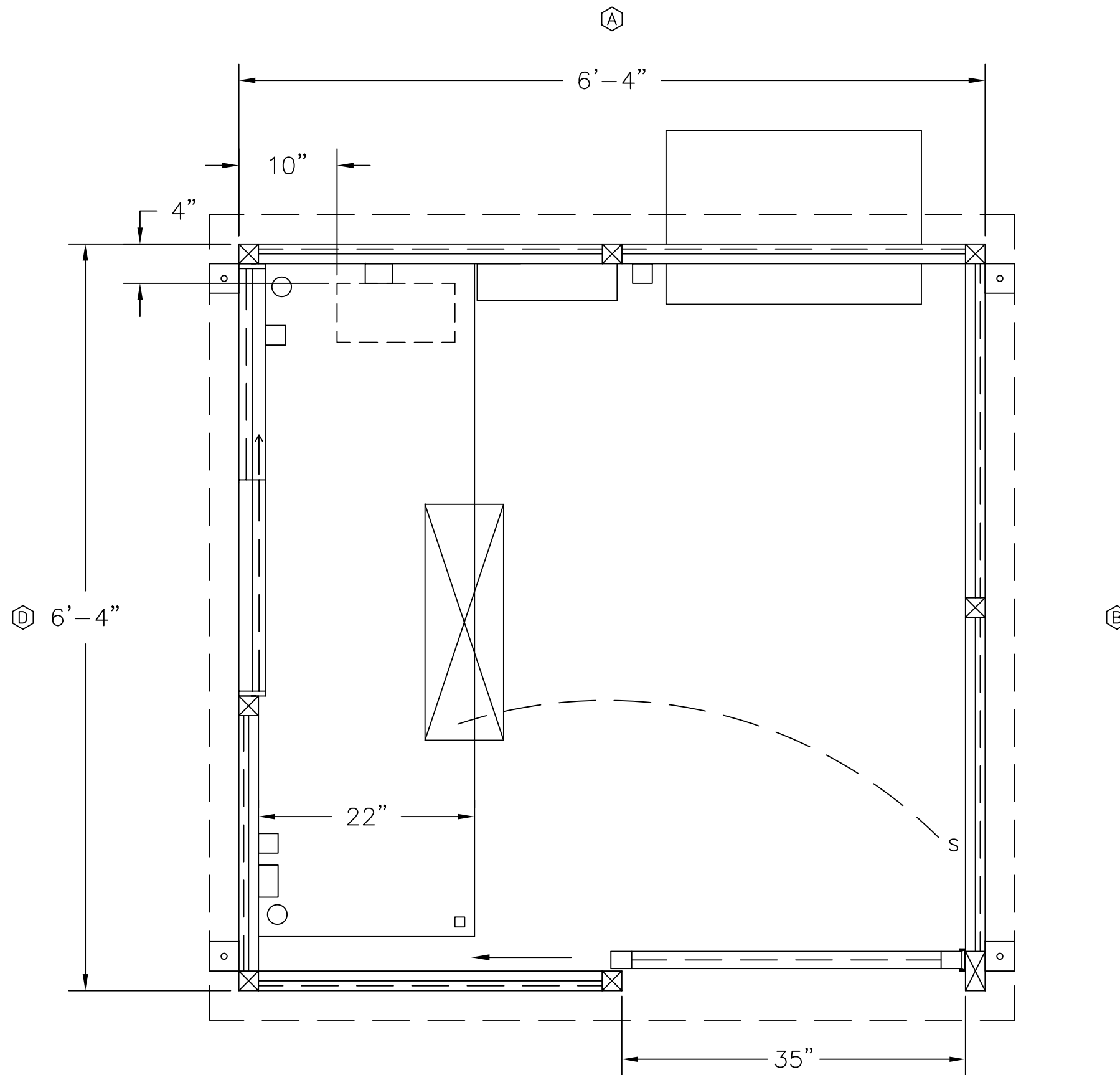
PLAN VIEW
