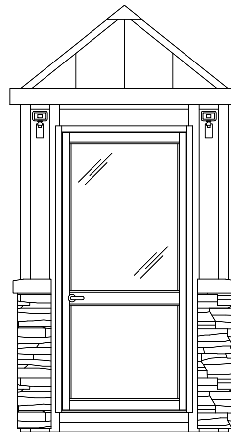
ELEVATION D
