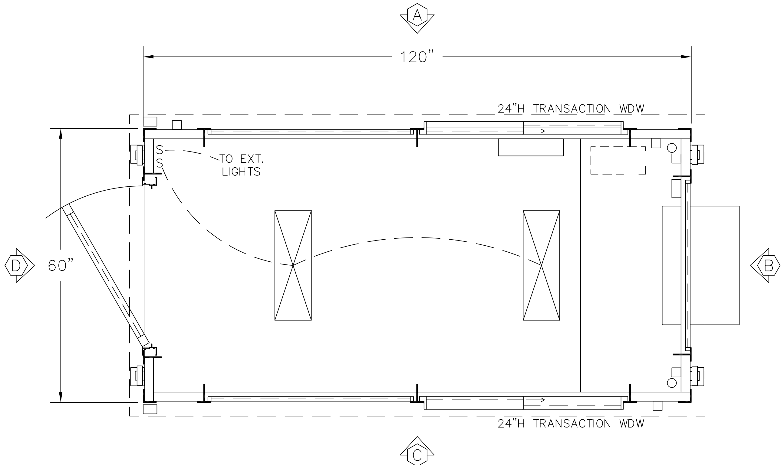
PLAN VIEW
