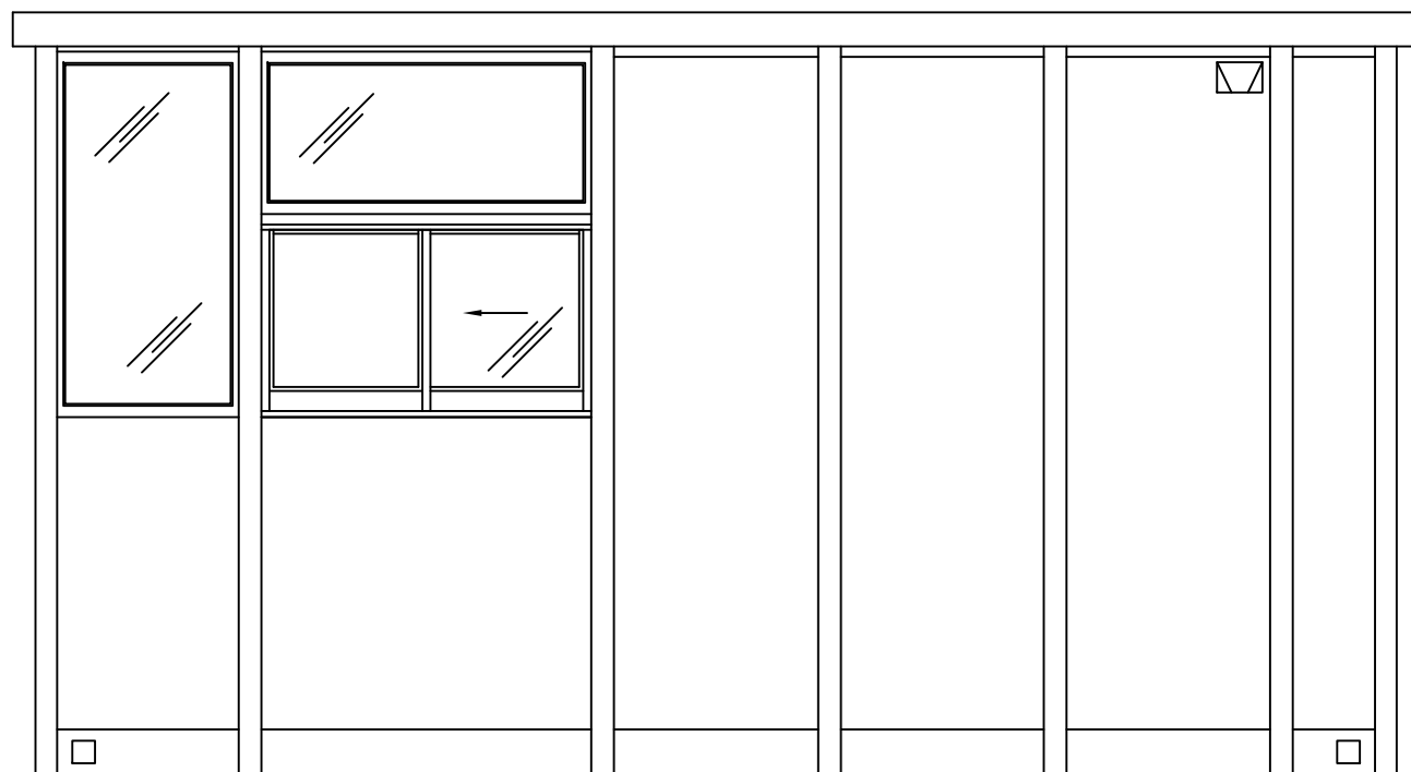
ELEVATION C
