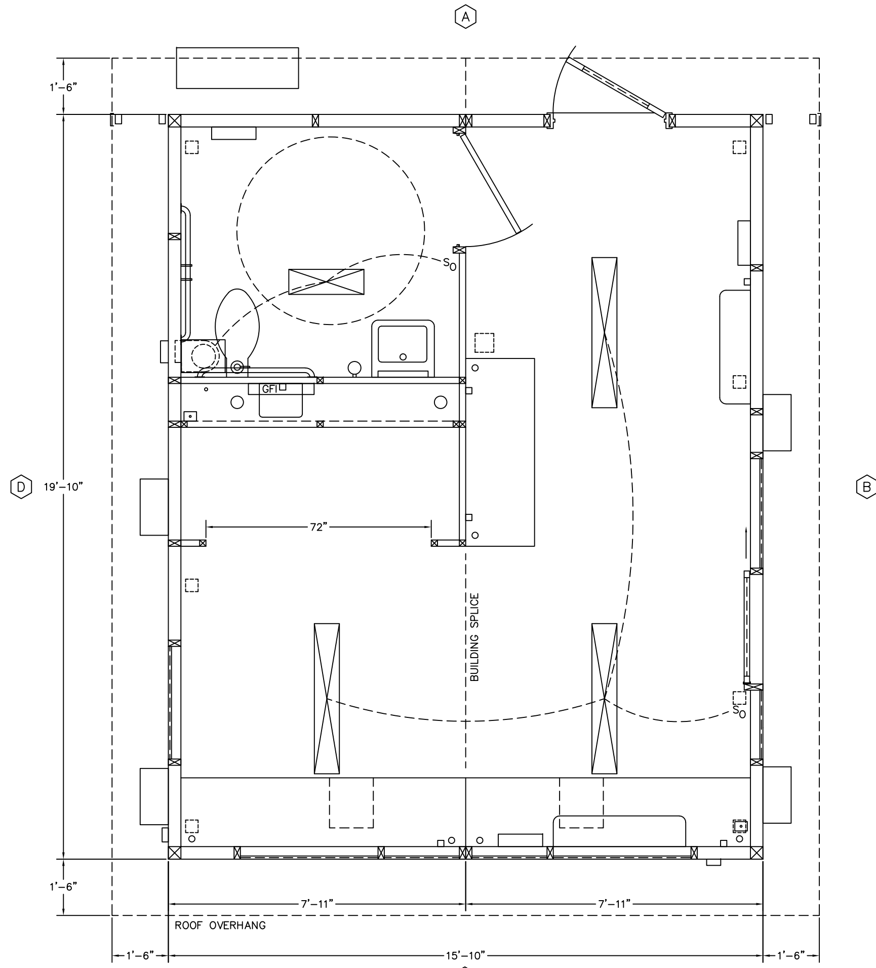
PLAN VIEW
